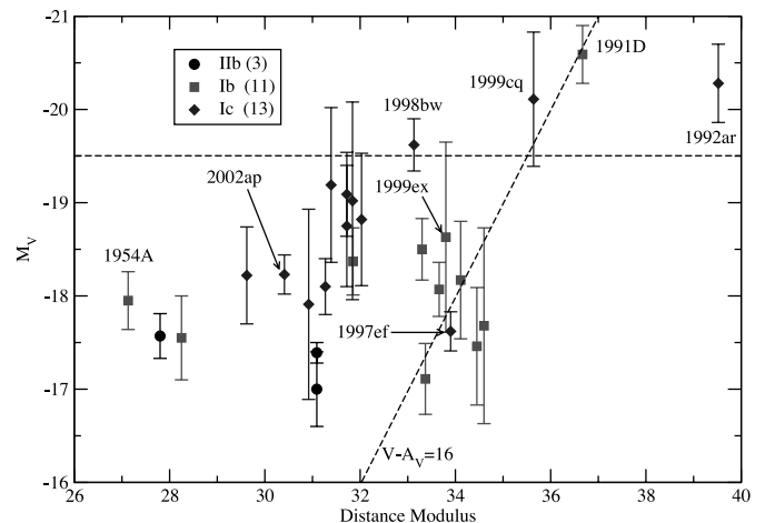
FIG. 1.—Absolute visual magnitude vs. distance modulus with the vertical error bars shown. Some key SNe are labeled. [See the electronic edition of the Journal for a color version of this figure.]
