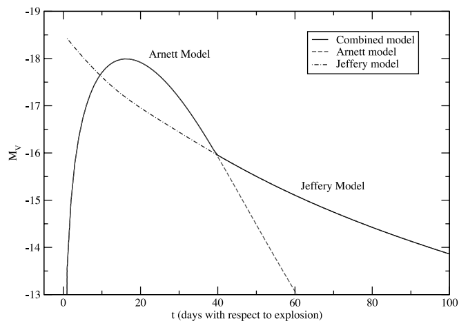
FIG. 7.—Combined model (solid line) and Arnett and Jeffery models (dashed lines). [See the electronic edition of the Journal for a color version of this figure.]
