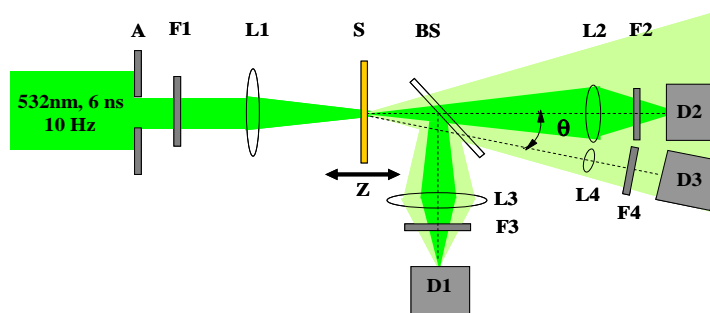
Fig. 1. Schematic of the Z scan set up for recording the nonlinear absorption and scattering. A - aperture, S - sample, F1, F2, F3, F4 - Neutral Density Filters, D1, D2, D3 - Detectors, BS - Beam splitter, L1, L2, L3, L4 - lens.
