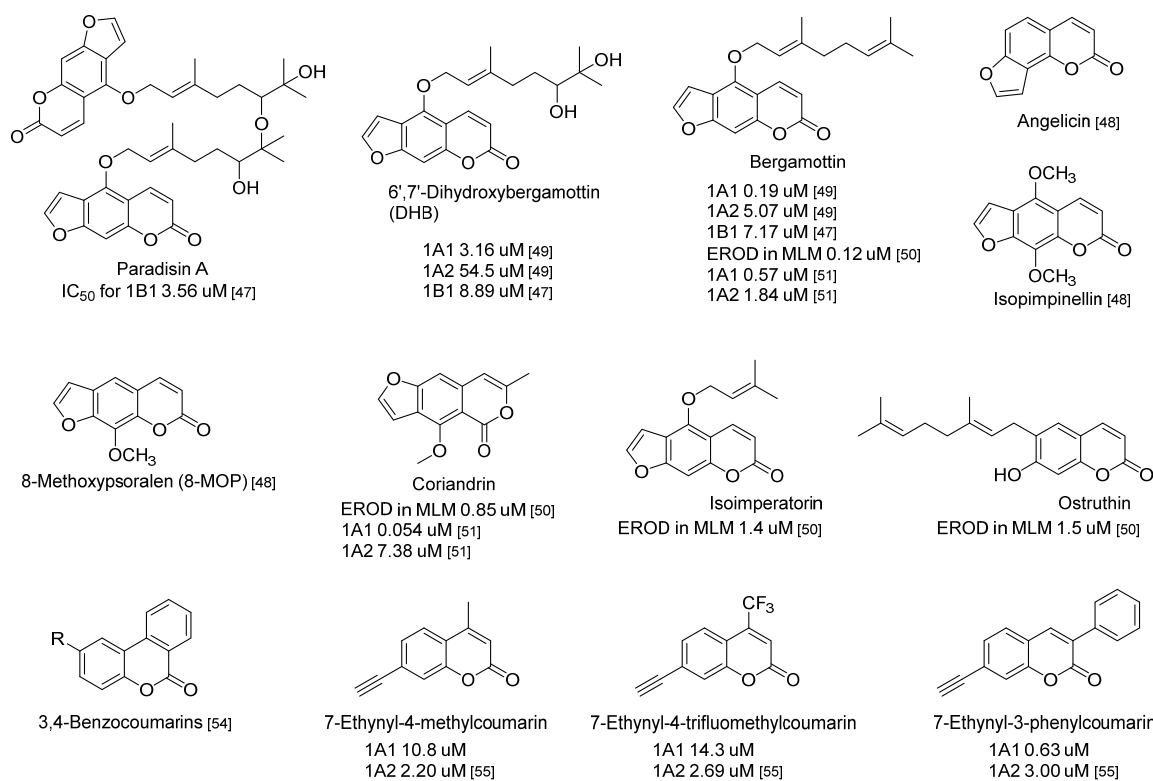
Figure 5. Coumarin derivatives as P450 family 1 inhibitors (MLM, mice liver microsome).
